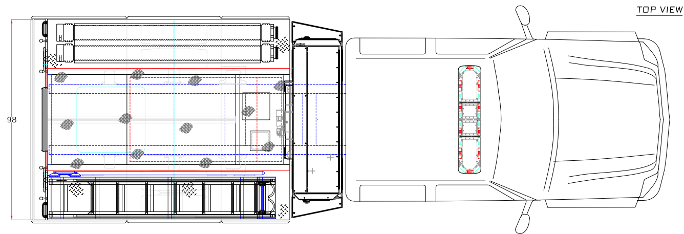
TOP VIEW
